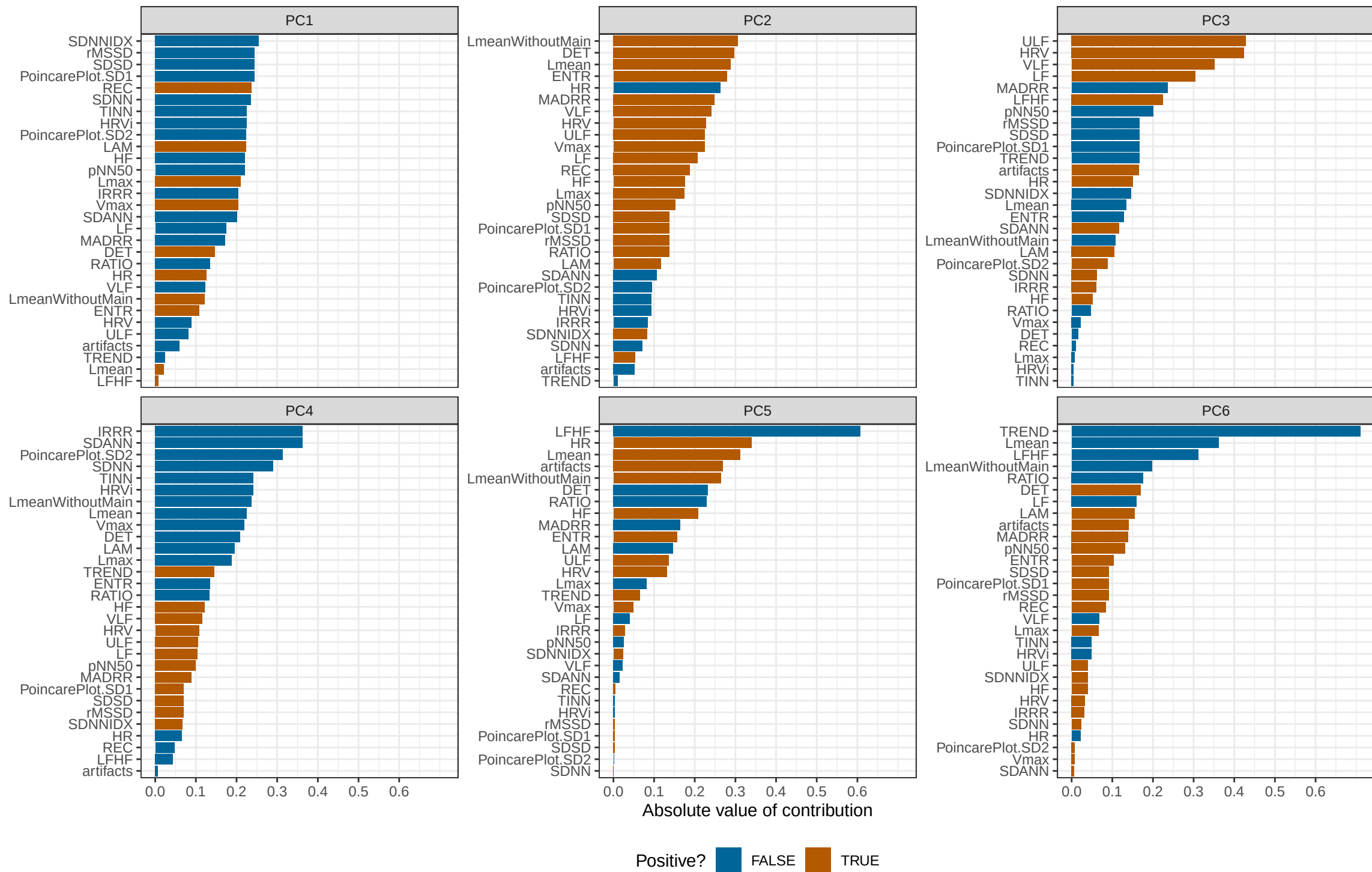
Loadings plot of the first 6 principal components of PCA for FLARE011
